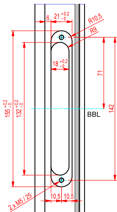
detail A (1 : 2)
