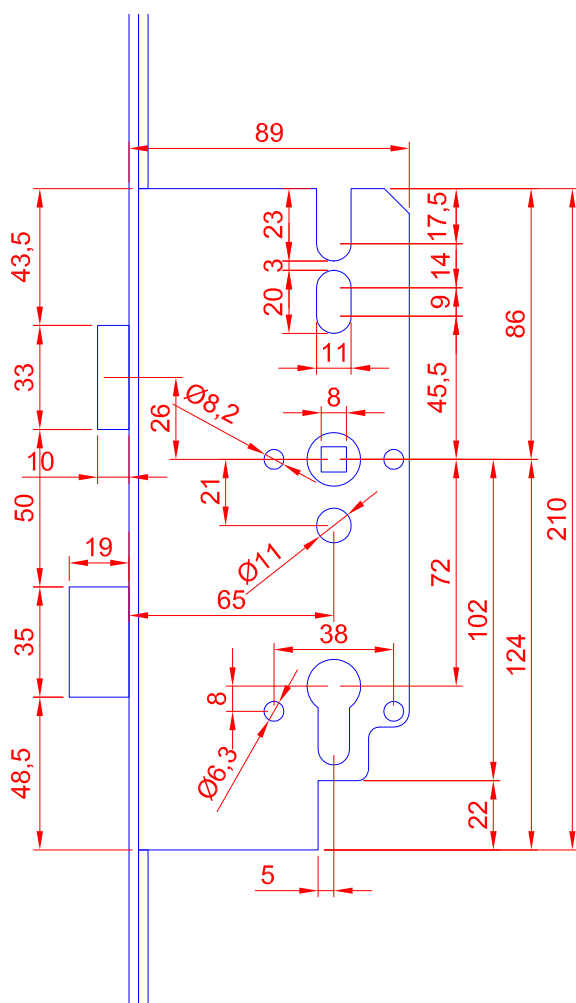
zámek GENIUS KVV AS2602 EA, EB (2600_1)
